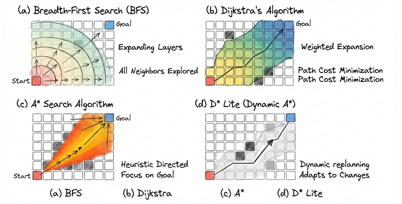
Fig 2.2: Search progression comparison of BFS, Dijkstra, A*, and D* Lite.
